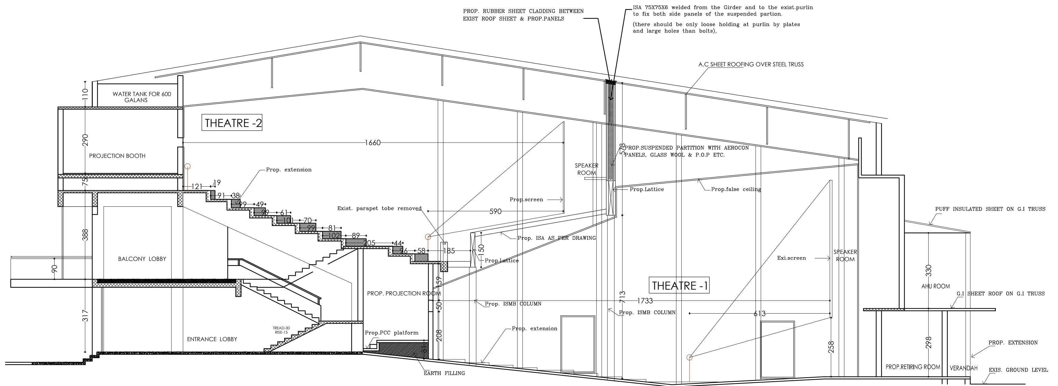
SECTION XX
